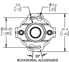
SC Mount*
