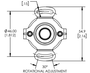
SF Mount
